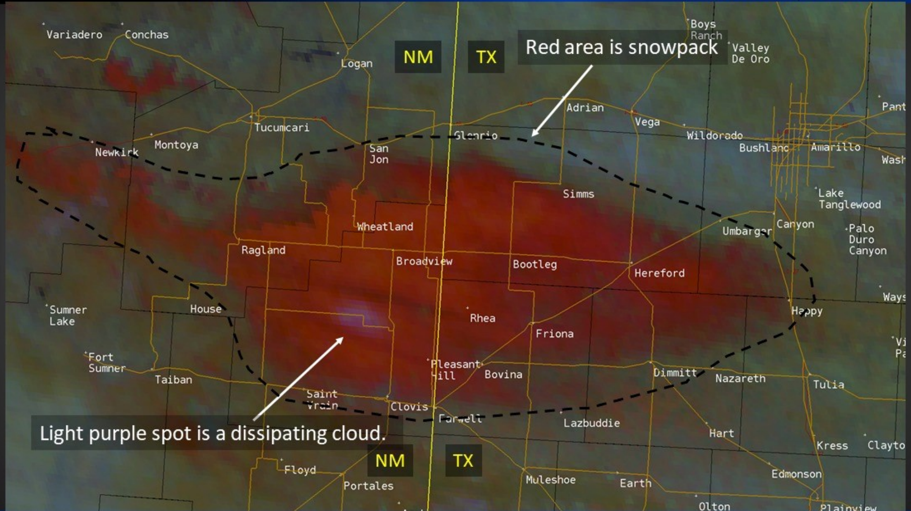
GOES-16 Satellite (Day Snow-Fog Product)
