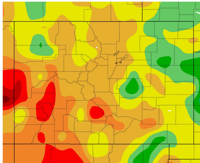
Departure from Normal Temperature (F) 8/1/2025 – 8/31/2025
