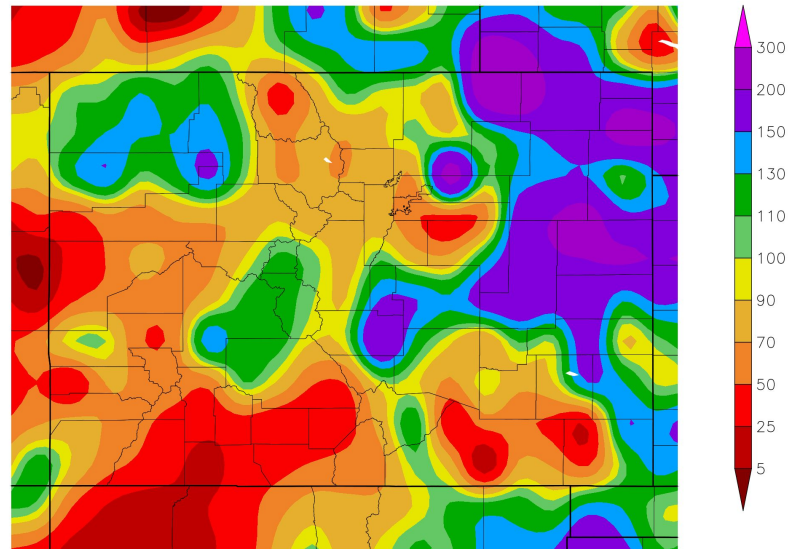
Percent of Normal Precipitation (%) 8/1/2025 – 8/31/2025
