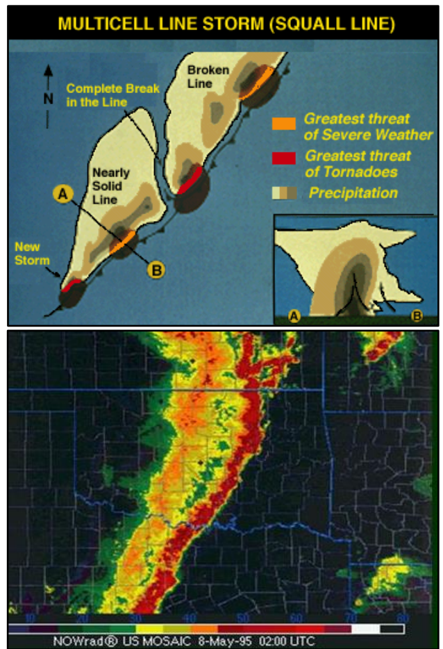
Figure 2. Schematic view of a multi-cell line storm (top) and associated radar signature (bottom) (National Weather Service)
