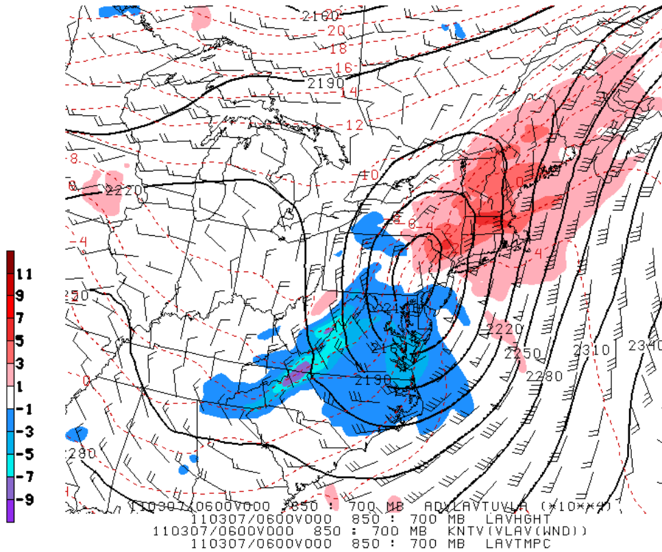
Figure 10. The 850-700mb layer averaged geopotential heights (m, black lines), temperatures (C, red dashed lines), winds (kts, barbs), and temperature advection (color filled, C km^{-1} 10^{-4} ) at 07/06 UTC from the NARR. [Click for image loop]
