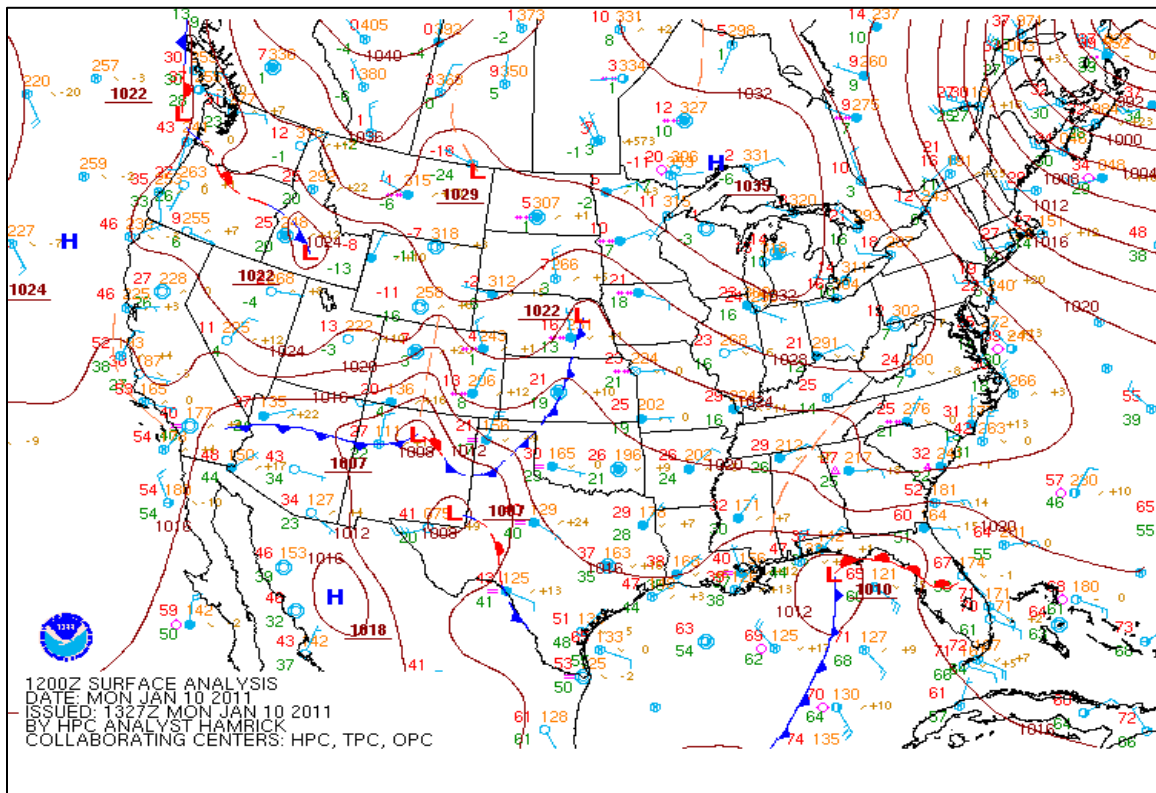
Figure 8. Surface analysis valid 1200 UTC 10 January 2011 (NWS Weather Prediction Center archive).
