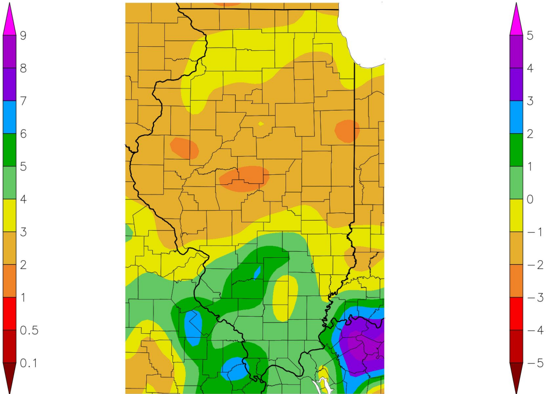
Departure from Normal Precipitation (in) 10/1/2025 – 10/31/2025
