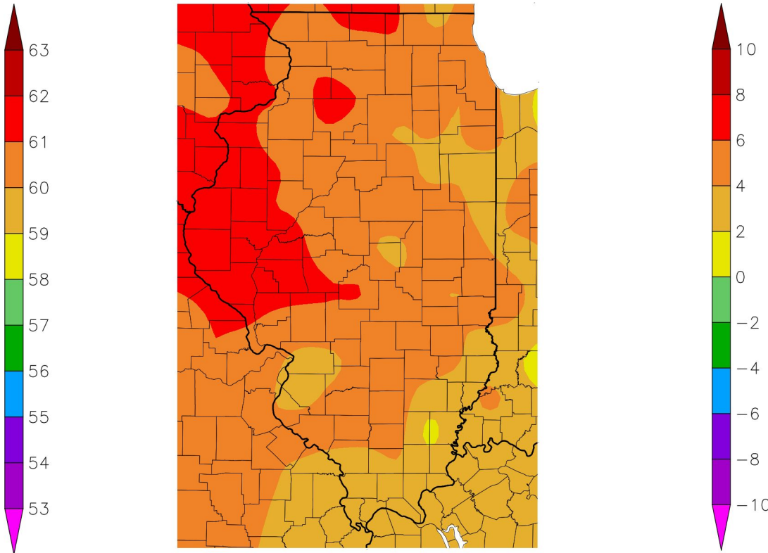
Departure from Normal Temperature (F) 10/1/2025 – 10/31/2025
