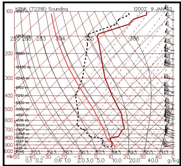
Fig. 7. Blacksburg, VA (KRNK) rawinsonde for 12 UTC 9 Jan 2003. Temperatures are in °C and winds are in knots. Location of KRNK is shown in Fig. 1. Courtesy of Plymouth State College.
