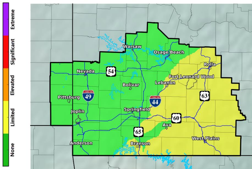
Severe Thunderstorms Risk Valid: 04/10/2017 02:00 AM - 04/11/2017 07:00 AM CDT
