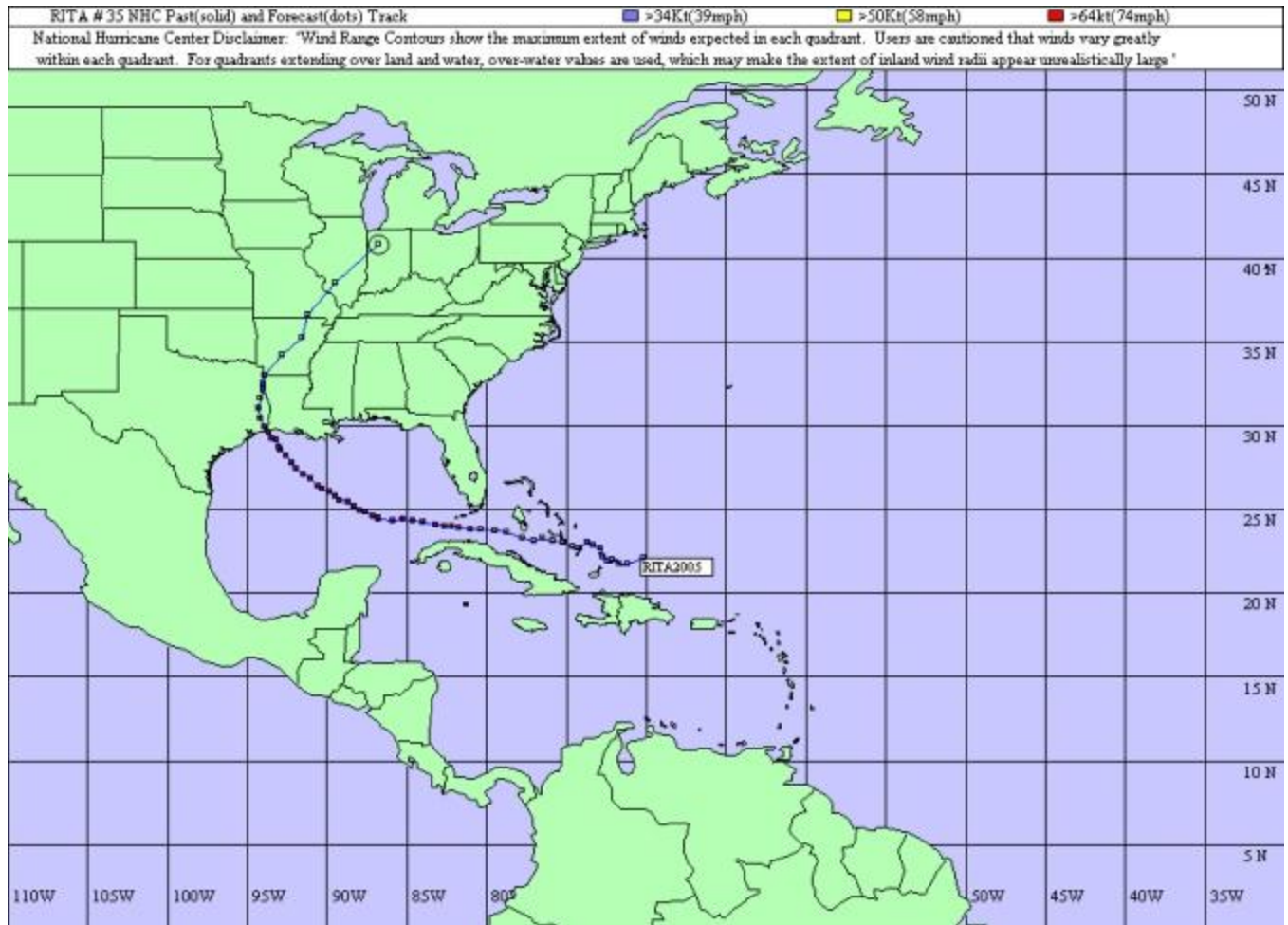
Rita Track
