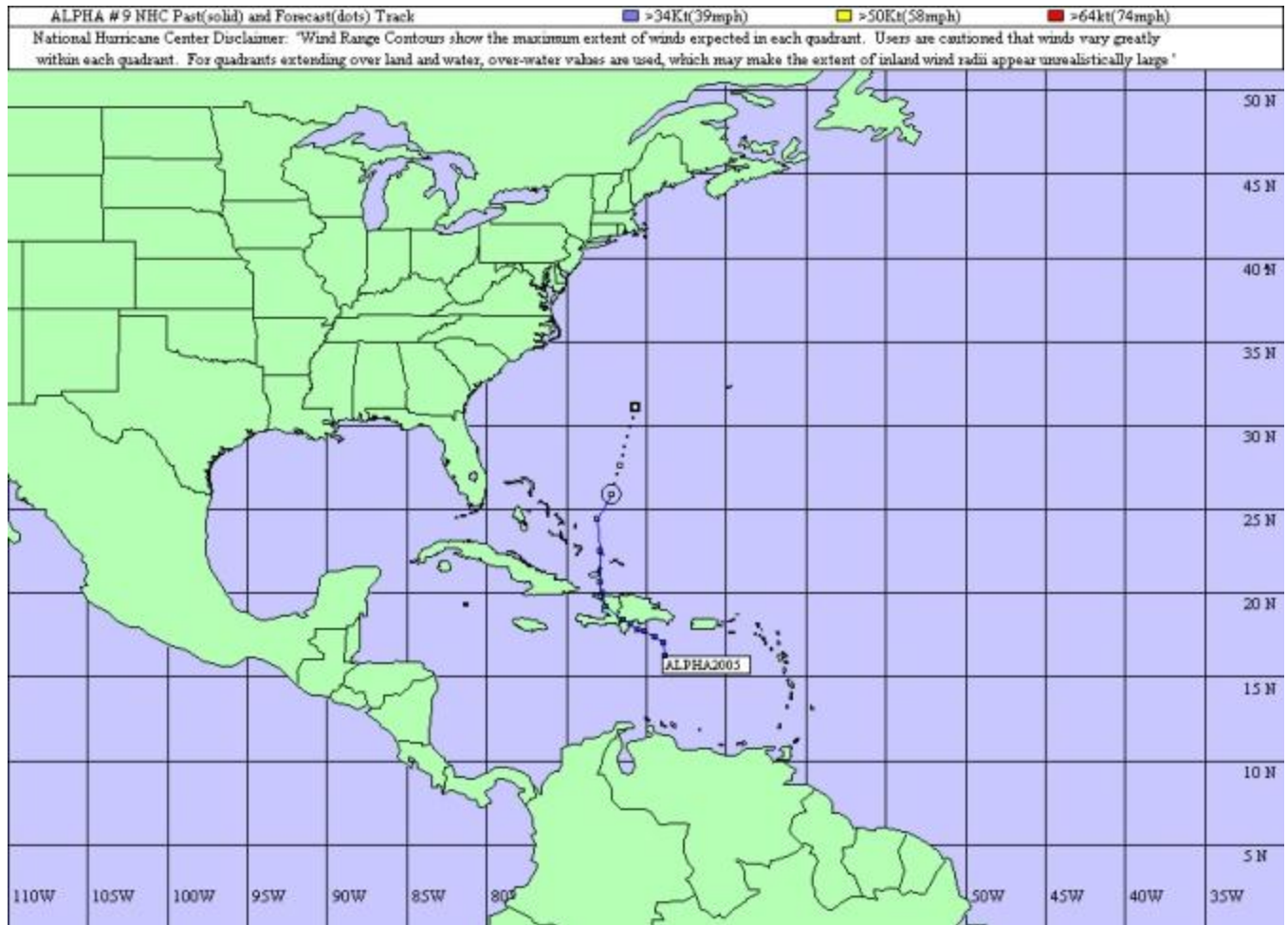
Alpha Track
