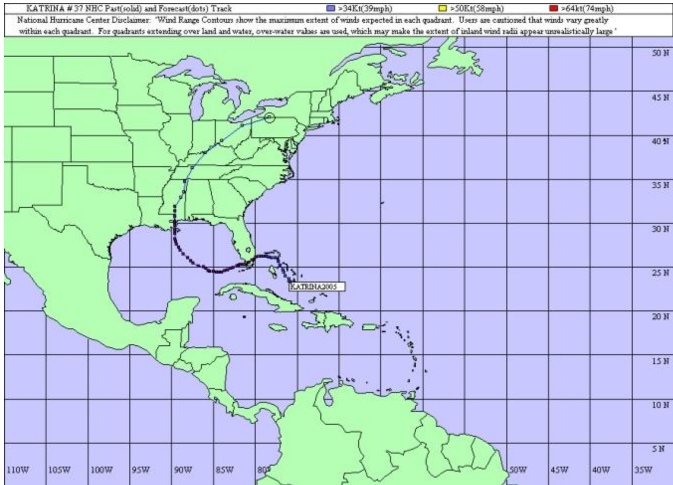
Katrina Track
