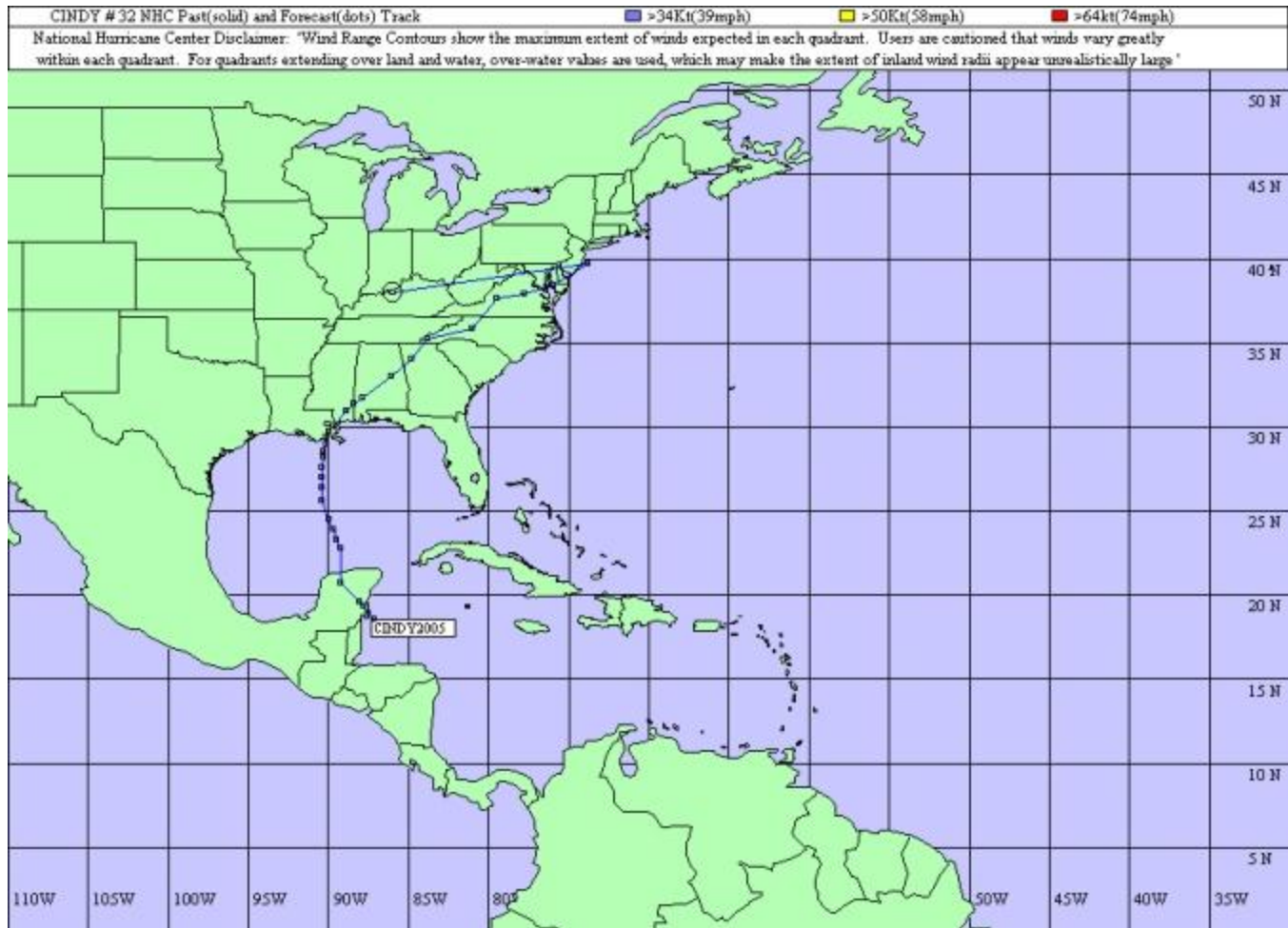
Cindy Track
