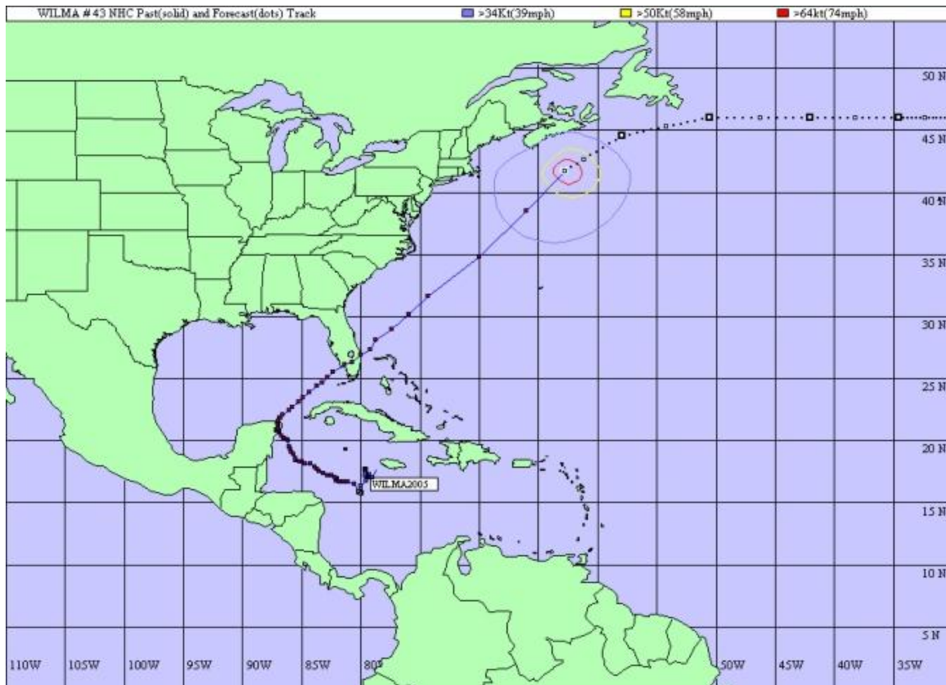
Wilma Track
