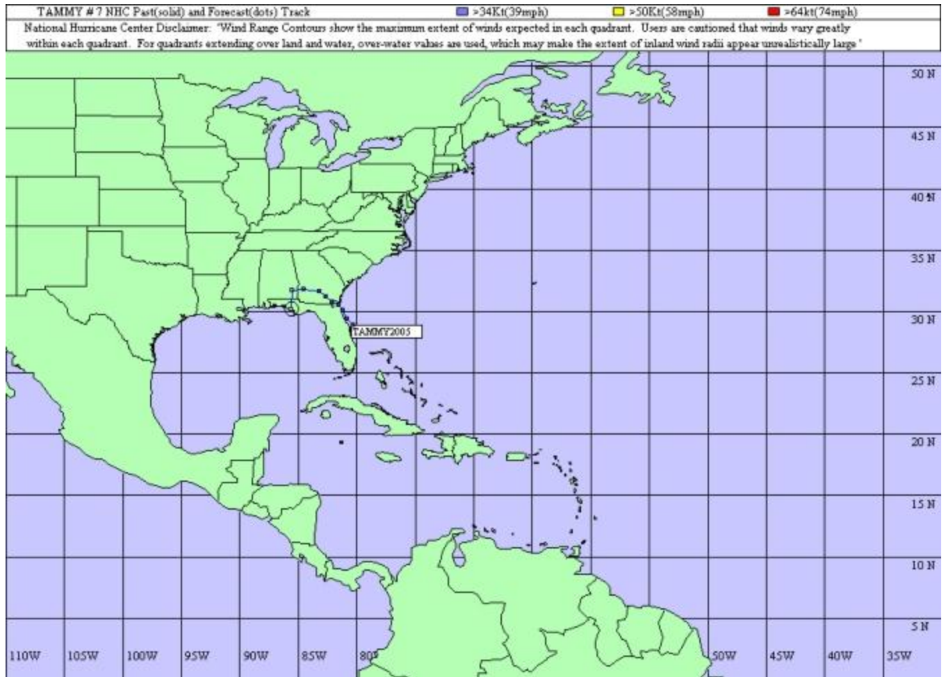
Tammy Track
