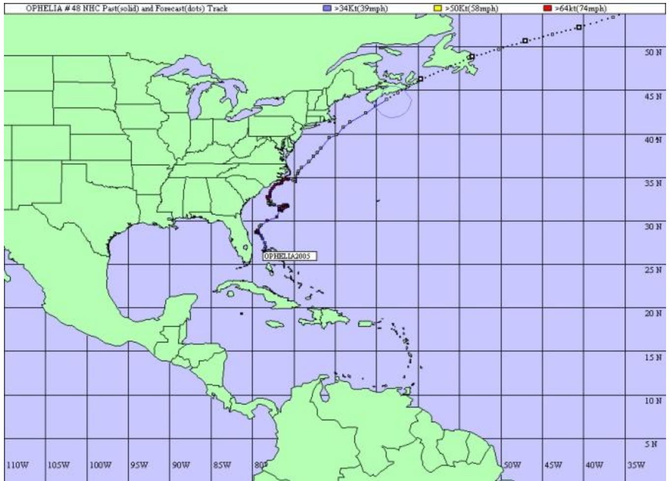
Ophelia Track
