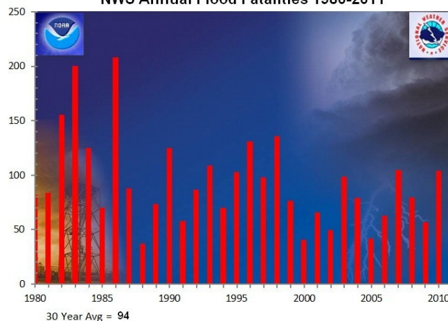
NWS Annual Flood Fatalities 1980-2011
