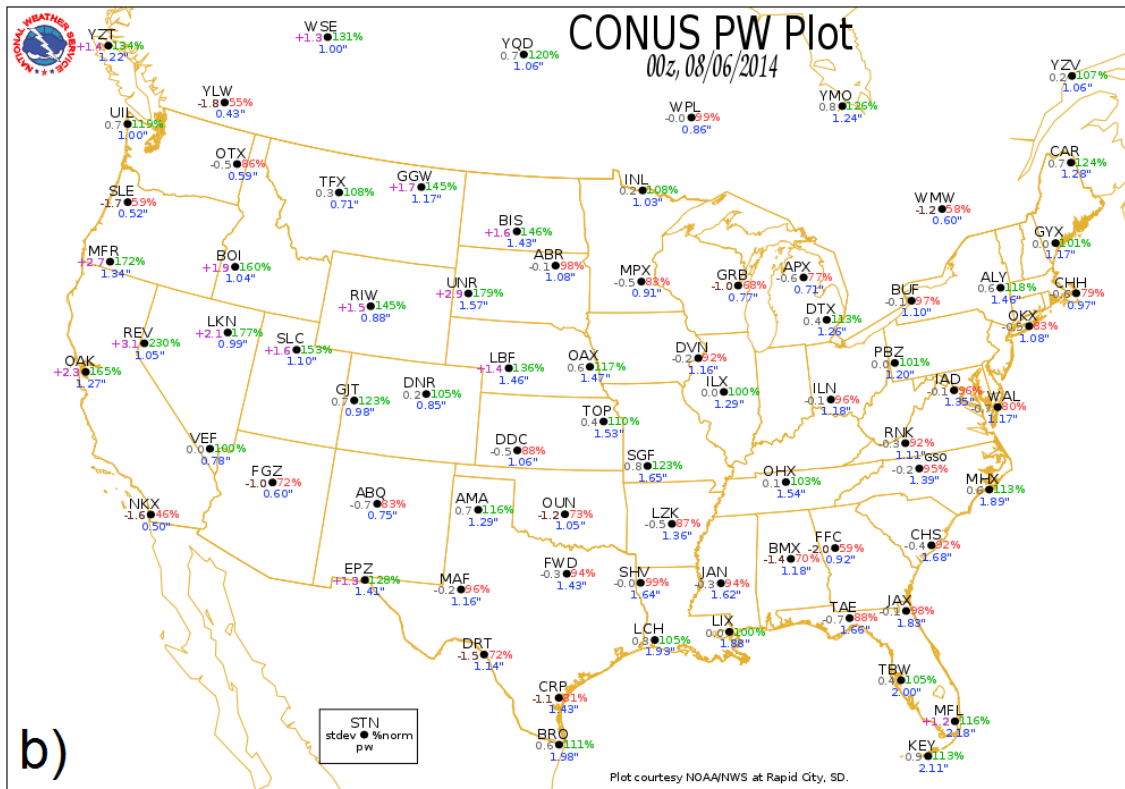
Figure 8. (a) Surface-to-300-mb precipitable water (in) for 6 am (or 1200 UTC) 5 August 2014. Station legend is given at the lower left. Refer to www.crh.noaa.gov/unr/?n=pw for information on the climatology used for these charts. (b) as in (a) but for 6 pm 5 August 2014 (or 0000 UTC 6 August 2014). These figures were produced with GrADS ( iges.org/grads/ ).
