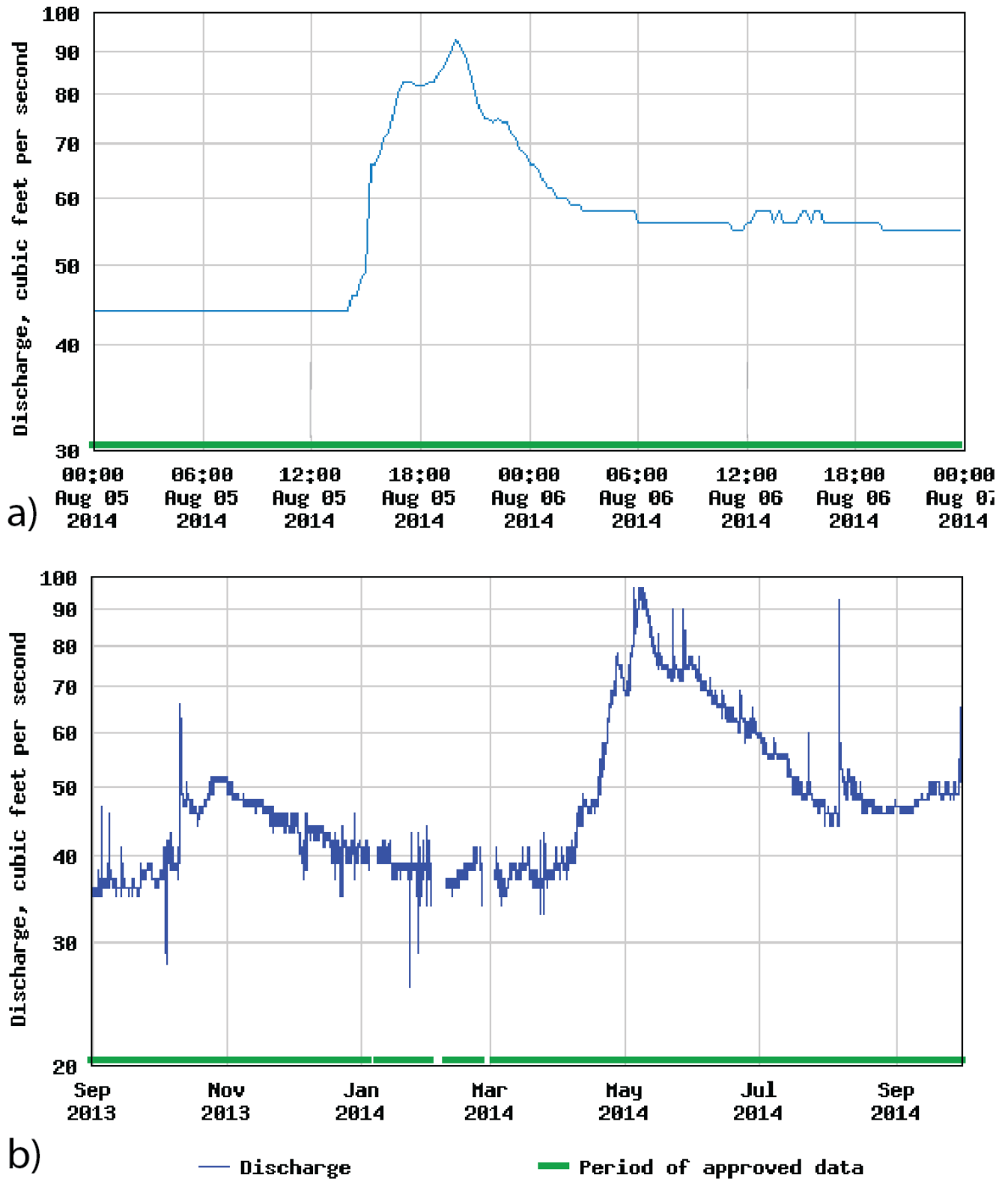
Figure 2. Hydrographs for USGS stream gage 06430770, Spearfish Creek near Lead, SD: (a) short-term hydrograph showing hydrologic response for 5–6 August 2014; and (b) longer-term hydrograph for 1 September 2013 through September 30 2014. Click image for an external version; this applies to all figures hereafter.
