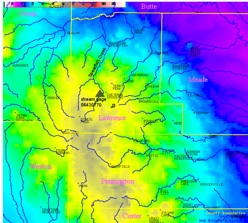
Figure 3. Major streams and topography for the northern Black Hills area with the location of interest indicated by a black “D” in Lawrence County and stream gage by the gray filled triangle. Elevation (ft) is given per the scale at upper left. Major streams are indicated by the blue lines, towns are in black, county names are in purple, and county lines are in yellow.
