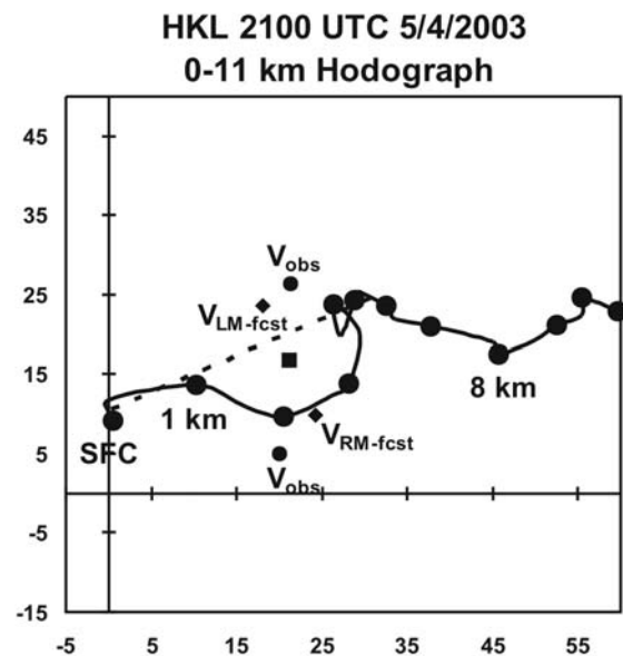
Figure 5. Hodograph derived from the Haskell, Oklahoma wind profiler valid at 2100 UTC 4 May 2003. Data are plotted every 500 m AGL, and filled circles are at every 1 km AGL (units are \text{m s}^{-1} ). The observed storm motions are plotted for the left- ( V_{\text{obs}} ) and right-
