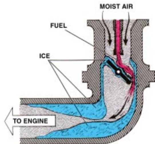
Figure 2-67. Carburetor Icing.
