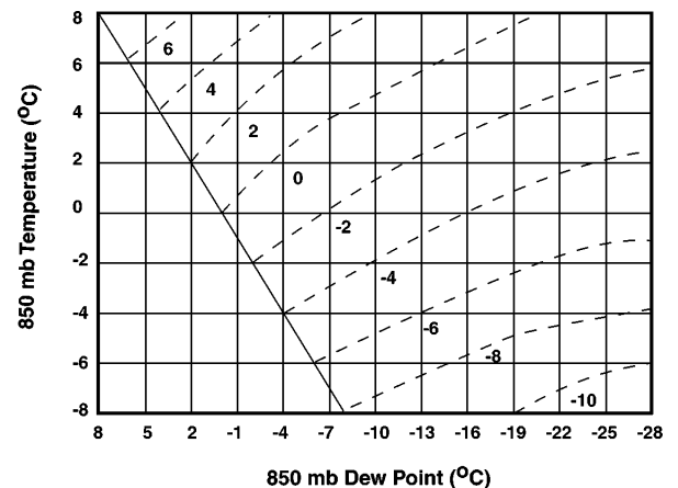
Figure 1-23. Computation of Wet-bulb Temperature at 1000 mb. Use this figure to compute 1000-mb wet-bulb temperature.
