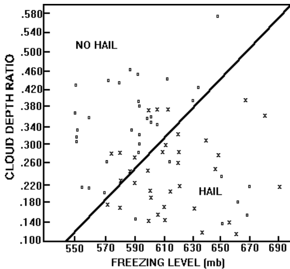
Figure 3-17. Hail Prediction Chart. See text. Also shown are the results of the original study.
