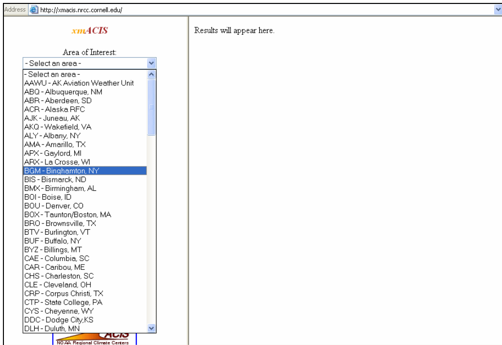
Fig. 1.1 xmACIS showing the "Area of Interest" list of WFOs.
