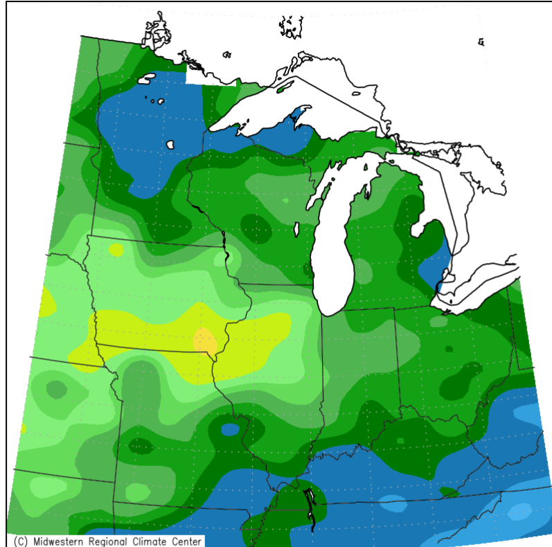
Accumulated Precipitation (in) August 1, 2020 to August 31, 2020
