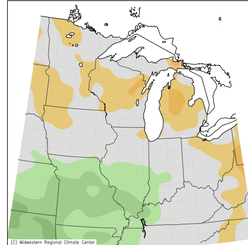
Average Temperature (°F): Departure from Mean August 1, 2020 to August 31, 2020
