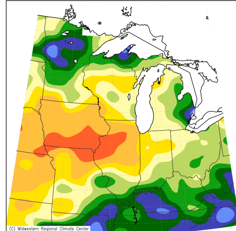
Accumulated Precipitation: Percent of Mean August 1, 2020 to August 31, 2020
