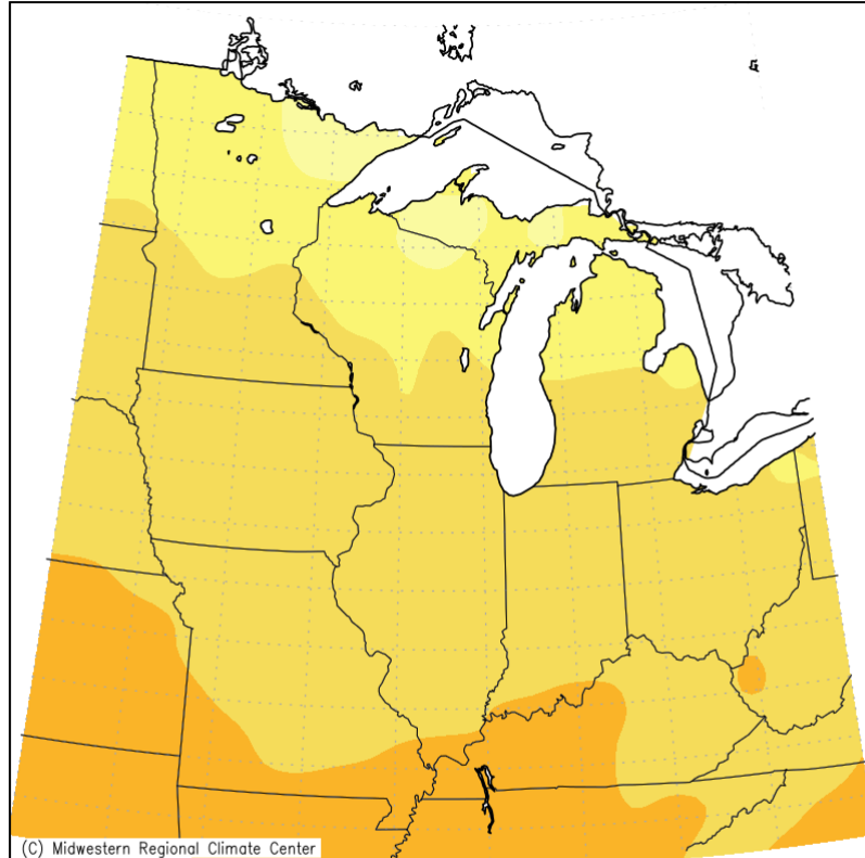
Average Temperature (°F) August 1, 2020 to August 31, 2020
