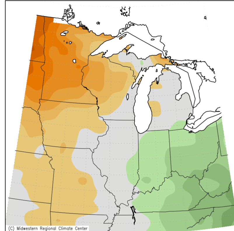
Average Temperature (°F): Departure from Mean June 1, 2023 to June 30, 2023
