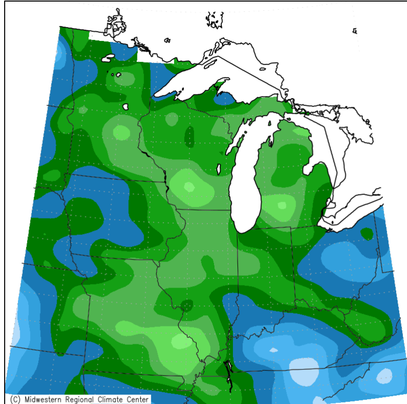
Accumulated Precipitation (in) June 1, 2023 to June 30, 2023
