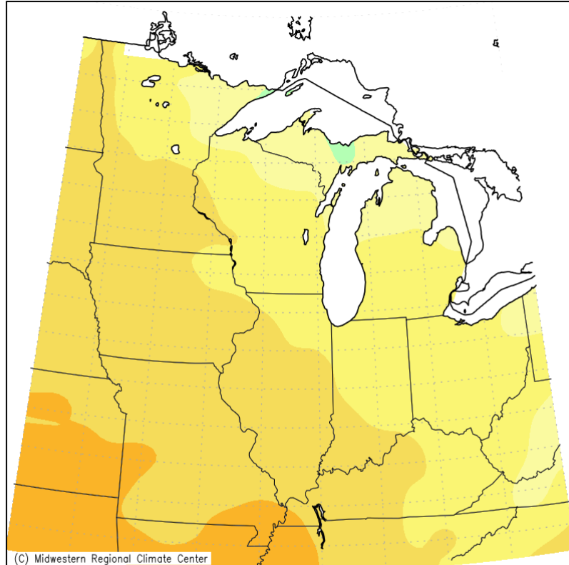
Average Temperature (°F) June 1, 2023 to June 30, 2023
