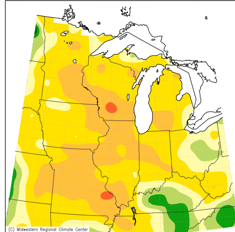
Accumulated Precipitation: Percent of Mean June 1, 2023 to June 30, 2023
