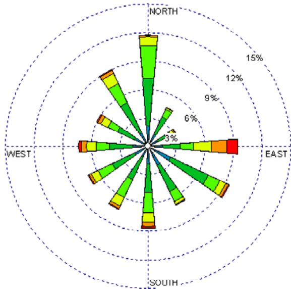
Albuquerque Int'l Airport (23050) 1985-2005 Annual Average - All Hours Average Speed = 7.18 kt
