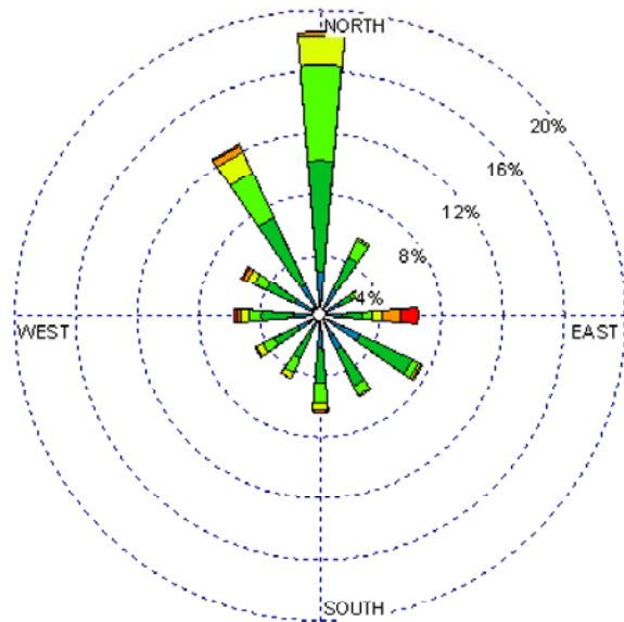
Albuquerque Int'l Airport (23050) 1985-2005 January - All hours Average Speed = 6.40 kt
