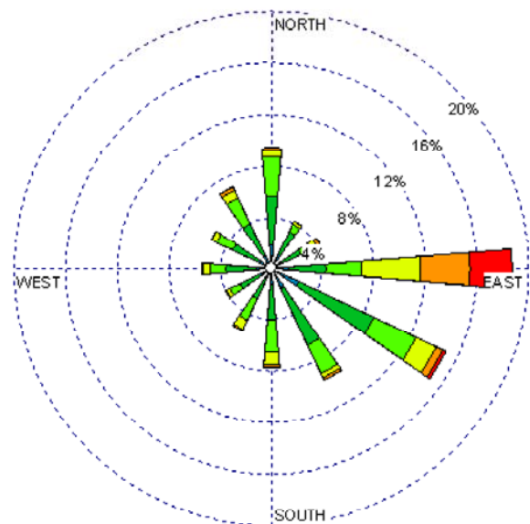
Albuquerque Int'l Airport (23050) 1985-2005 June - 03-09Z Average Speed = 8.20 kt
