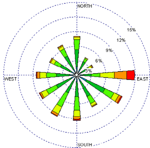
Albuquerque Int'l Airport (23050) 1985-2005 June - All hours Average Speed = 7.94 kt
