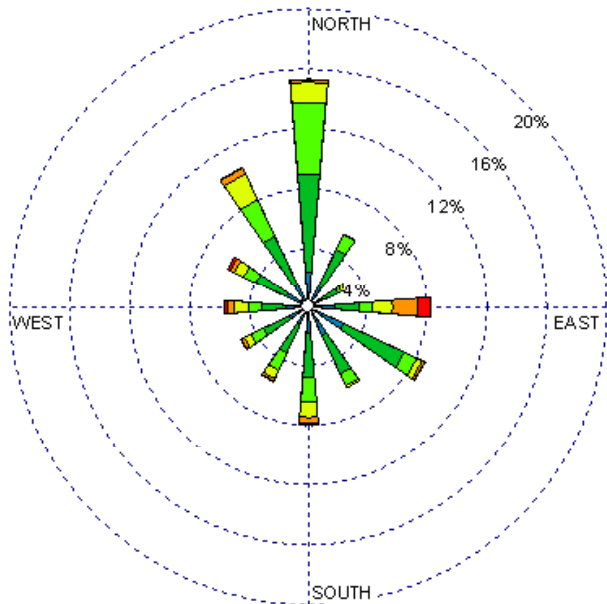
Albuquerque Int'l Airport (23050) 1985-2005 November - All hours Average - 6.8 kt
