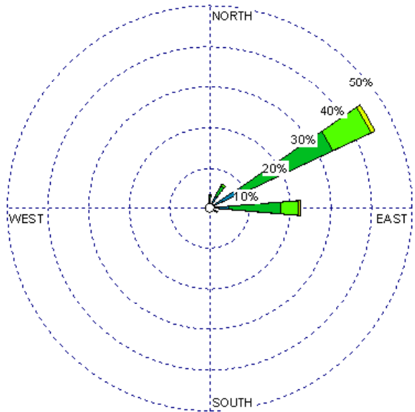
Farmington (23090) 1985-2005 August - 10-15z Average Speed - 5.06 kt
