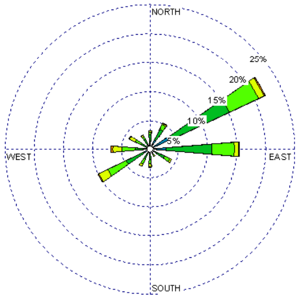
Farmington (23090) 1985-2005 August - All hours Average Speed - 5.94 kt
