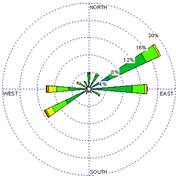
Farmington (23090) 1985-2005 December - All hours Average Speed - 4.93 kt
