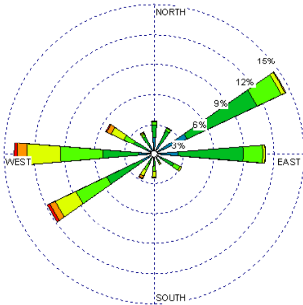
Farmington (23090) 1985-2005 February - All hours Average Speed - 5.81 kt
