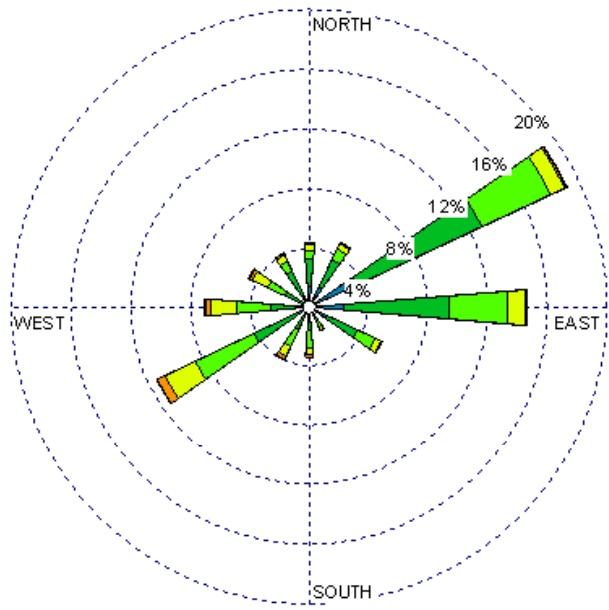
Farmington (23090) 1985-2005 July - All hours Average Speed - 6.55 kt
