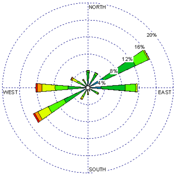
Farmington (23090) 1985-2005 November - All hours Average Speed - 5.99 kt
