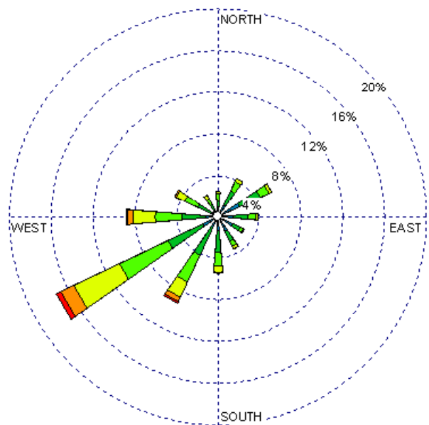
Gallup (23081) 1985-2005 Annual Average - all hours Average Speed = 5.81 kts
