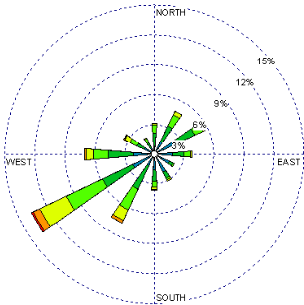
Gallup (23081) 1985-2005 December - All hours Average Speed - 4.25 kt
