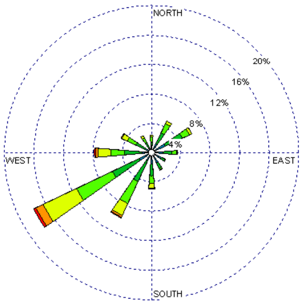
Gallup (23081) 1985-2005 February - All hours Average Speed - 5.56 kt
