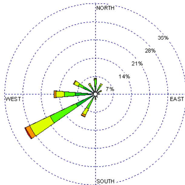
Gallup (23081) 1985-2005 January - 19-23z Average Speed - 8.23 kt
