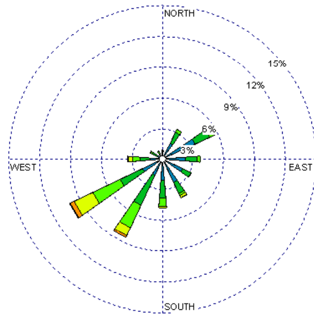
Gallup (23081) 1985-2005 January - 03-09z Average Speed - 3.12 kt
