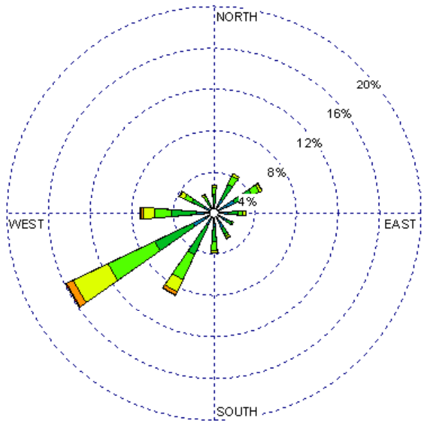
Gallup (23081) 1985-2005 January - All hours Average Speed - 4.56 kt
