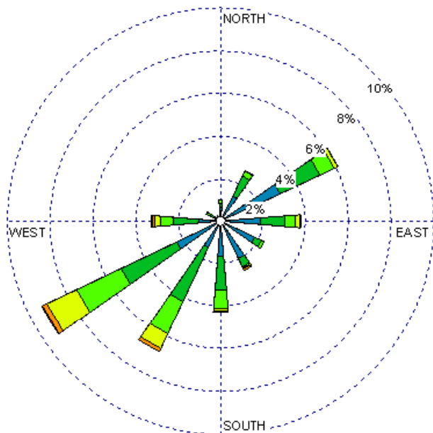
Gallup (23081) 1985-2005 January - 10-15z Average Speed - 2.69 kt
