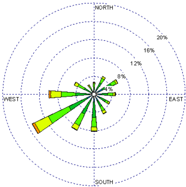
Gallup (23081) 1985-2005 July - All hours Average Speed - 5.90 kt
