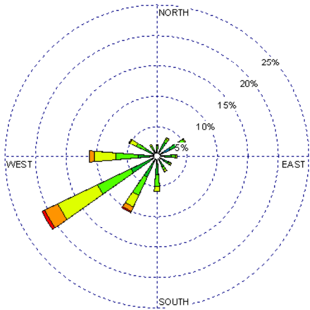
Gallup (23081) 1985-2005 June - All hours Average Speed - 6.86 kt
