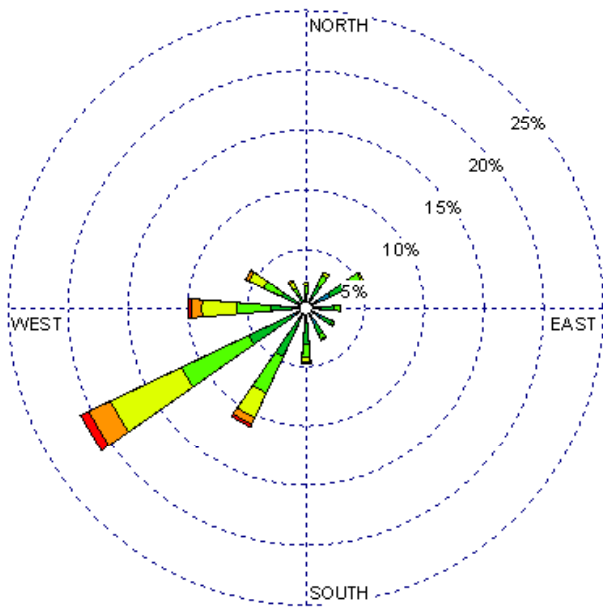
Gallup (23081) 1985-2005 March - All hours Average Speed - 6.71 kt
