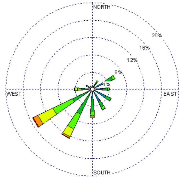
Gallup (23081) 1985-2005 March - 03-09z Average Speed - 4.56 kt
