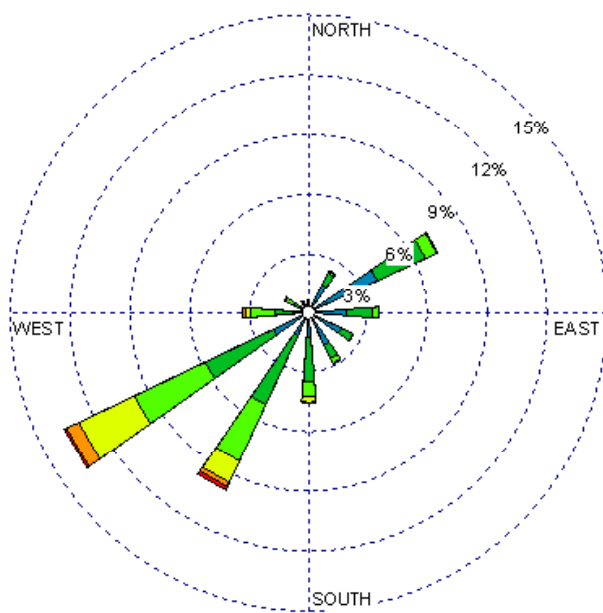
Gallup (23081) 1985-2005 March - 10-15z Average Speed - 3.62 kt
