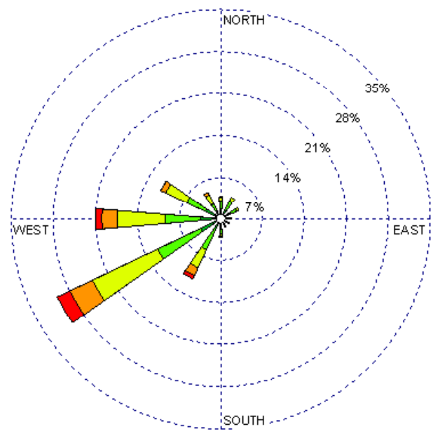
Gallup (23081) 1985-2005 March - 19-23z Average Speed - 11.24 kt
