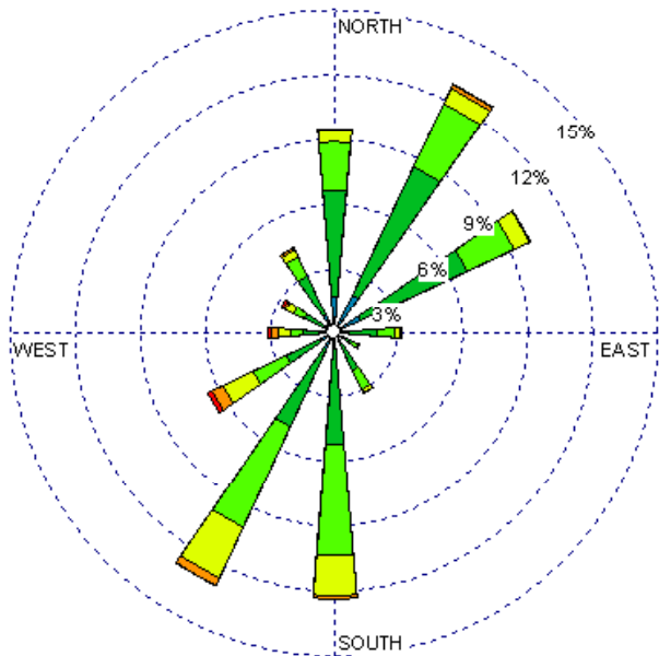
Las Vegas (23053) 1985-2005 Annual Average - 10 to 15Z Average Speed = 6.52 kts
