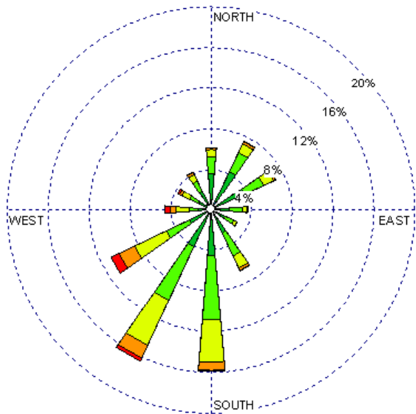
Las Vegas (23053) 1985-2005 Annual Average - all hours Average Speed = 8.91 kts
