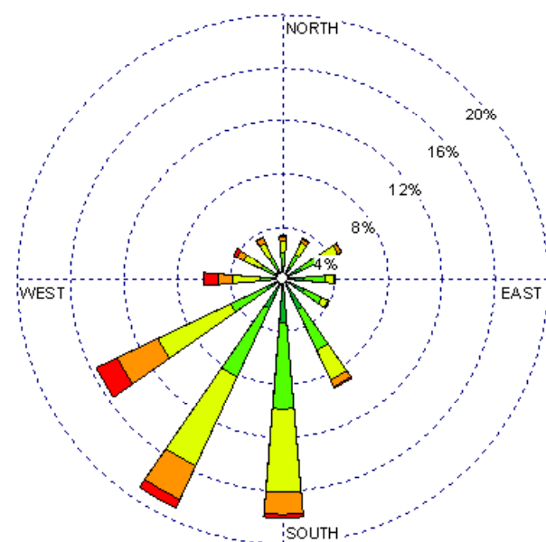
Las Vegas (23053) 1985-2005 Annual Average - 19 to 23Z Average Speed = 11.52 kts
