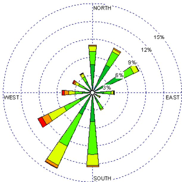
Las Vegas (23054) 1985-2005 April - 10-15z Average Speed - 7.49 kt Calms: 17.15%
