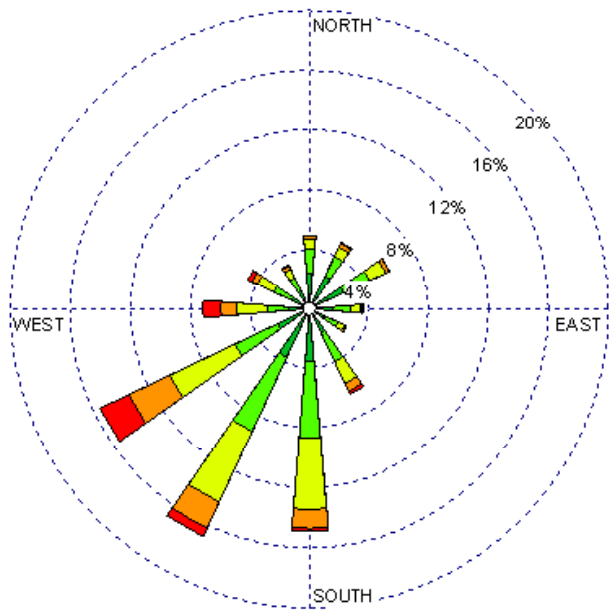
Las Vegas (23054) 1985-2005 April - All hours Average Speed - 10.36 kt Calms: 9.18%
