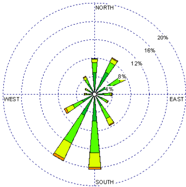
Las Vegas (23054) 1985-2005 August - All hours Average Speed - 7.61 kt
