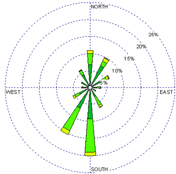
Las Vegas (23054) 1985-2005 August - 03-09z Average Speed - 6.72 kt
