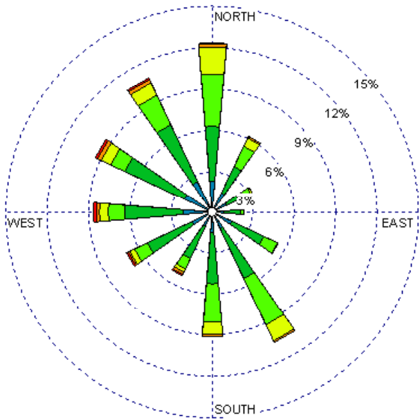
Roswell (23009) 1985-2005 December - All hours Average Speed - 6.48 kt
