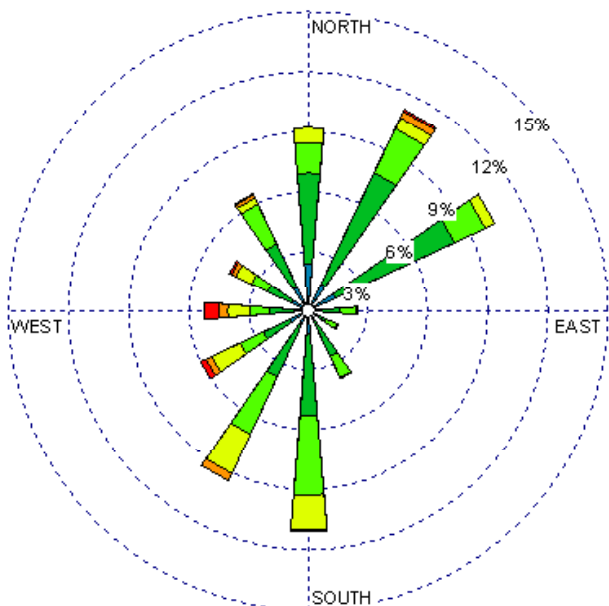
Las Vegas (23054) 1985-2005 January - 10-15z Average Speed - 6.44 kt
