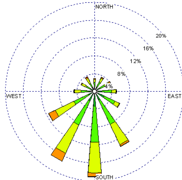
Las Vegas (23054) 1985-2005 July - 19-23z Average Speed - 10.37 kt
