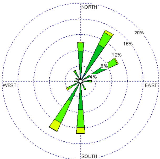
Las Vegas (23054) 1985-2005 July - 10-15z Average Speed - 5.56 kt
