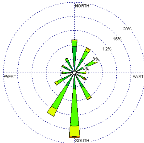
Las Vegas (23054) 1985-2005 July - 03-09z Average Speed - 7.11 kt
