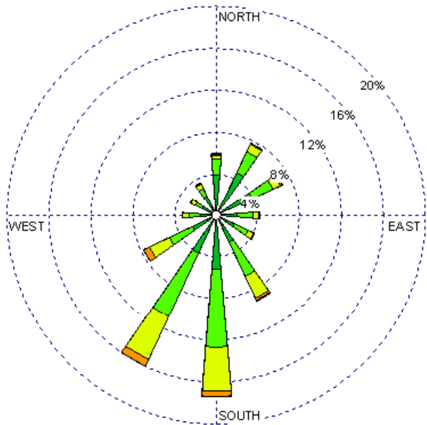
Las Vegas (23054) 1985-2005 July - All hours Average Speed - 7.95 kt
