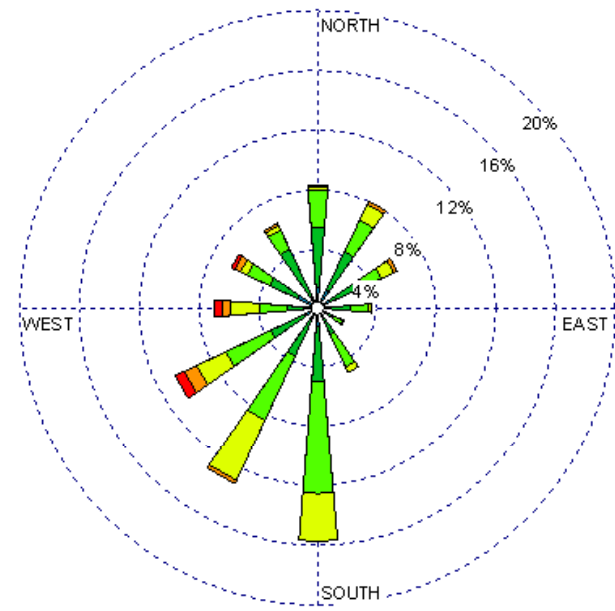
Las Vegas (23054) 1985-2005 March - 03-09z Average Speed - 8.08 kt
