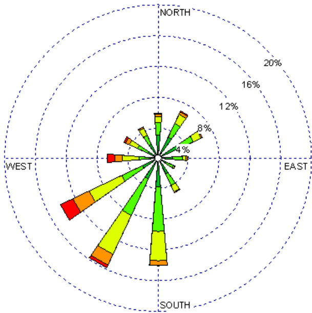
Las Vegas (23054) 1985-2005 March - All hours Average Speed - 9.72 kt
