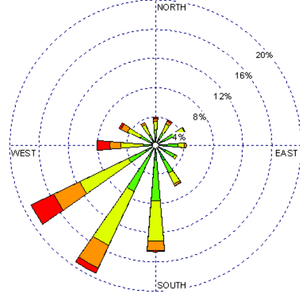
Las Vegas (23054) 1985-2005 March - 19-23z Average Speed - 12.39 kt
