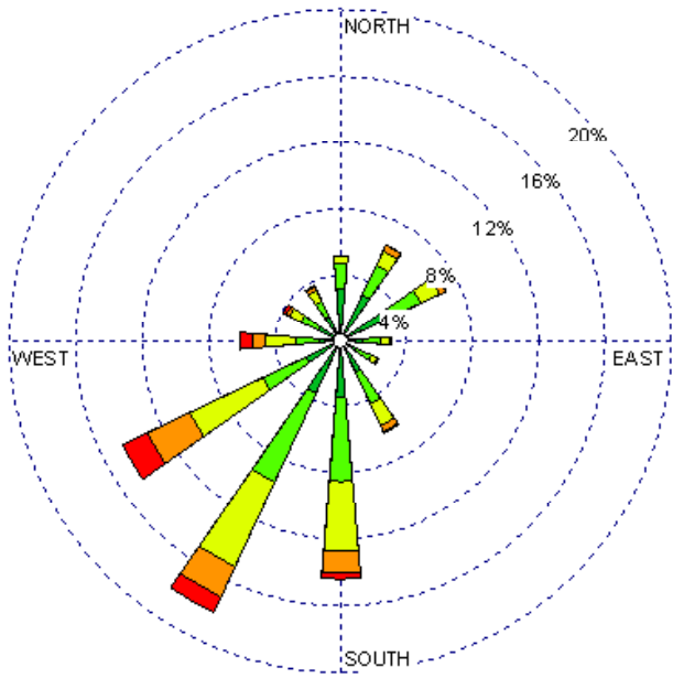
Las Vegas (23054) 1985-2005 May - All hours Average Speed - 10.05 kt
