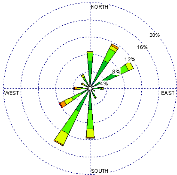
Las Vegas (23054) 1985-2005 May - 10-15z Average Speed - 6.86 kt
