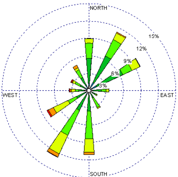
Las Vegas (23054) 1985-2005 November - 10-15z Average Speed - 7.07 kt
