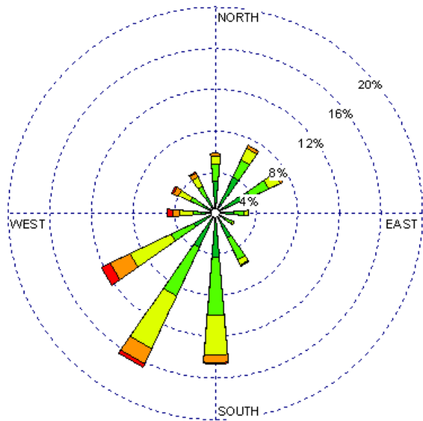
Las Vegas (23054) 1985-2005 November - All hours Average Speed - 9.09 kt
