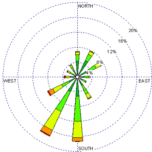
Las Vegas (23054) 1985-2005 October - All hours Average Speed - 8.42 kt
