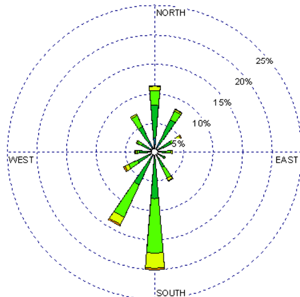
Las Vegas (23054) 1985-2005 October - 03-09z Average Speed - 6.72 kt
