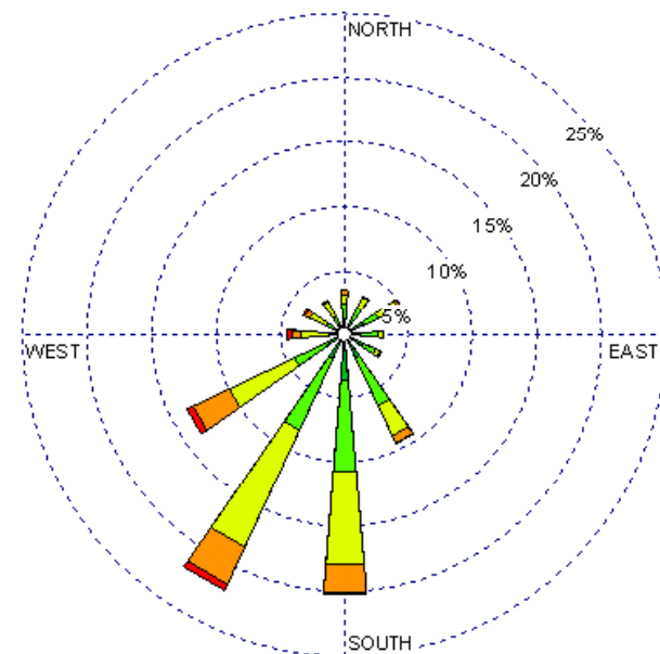
Las Vegas (23054) 1985-2005 October - 19-23z Average Speed - 11.15 kt
