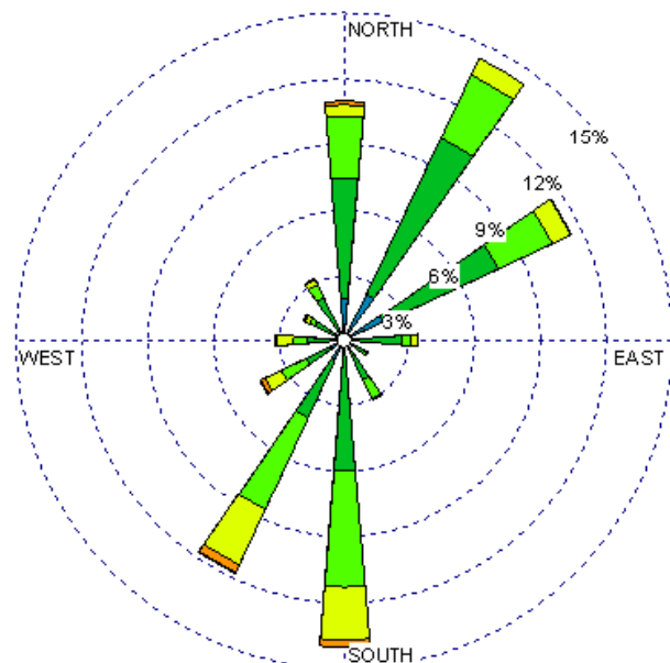
Las Vegas (23054) 1985-2005 October - 10-15z Average Speed - 6.33 kt
