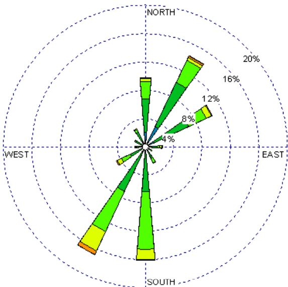
Las Vegas (23054) 1985-2005 September - 10-15z Average Speed= 6.33 kt
