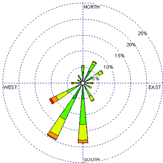
Las Vegas (23054) 1985-2005 September - All hours Average Speed= 8.80 kt
