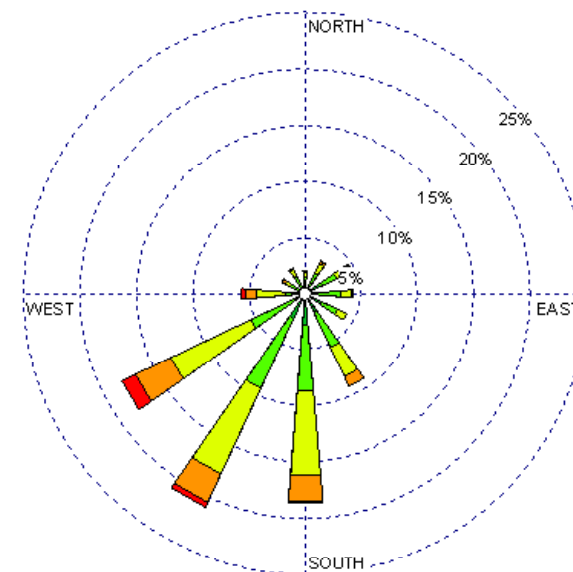
Las Vegas (23054) 1985-2005 September - 19-23z Average Speed= 11.49 kt
