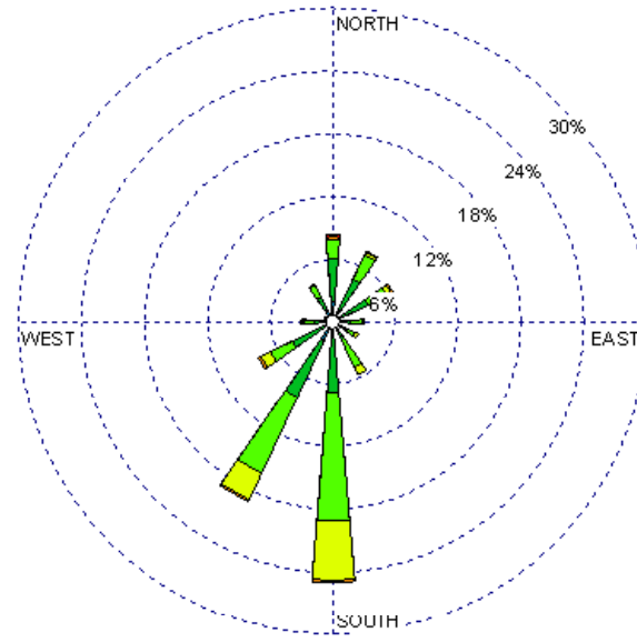
Las Vegas (23054) 1985-2005 September - 03-09z Average Speed= 7.54 kt
