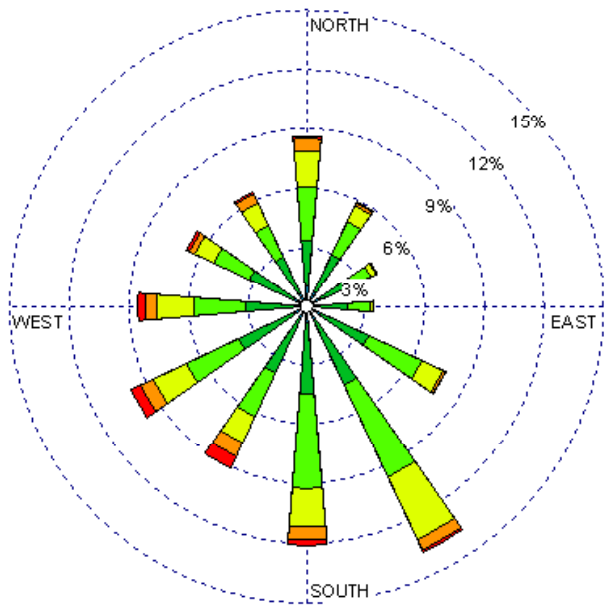
Roswell (23009) 1985-2005 April - All hours Average Speed - 8.98 kt
