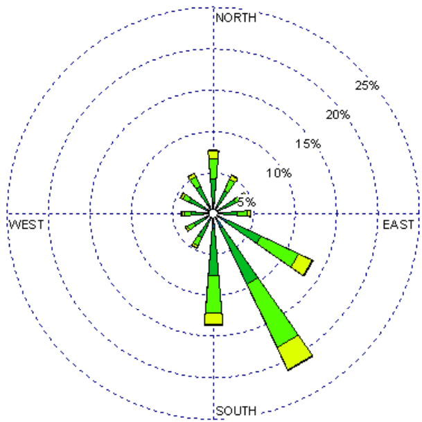
Roswell (23009) 1985-2005 August - All hours Average Speed - 6.97 kt
