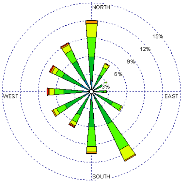
Roswell (23009) 1985-2005 November - All hours Average Speed - 6.93 kt
