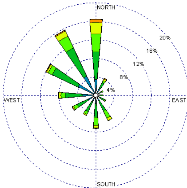
Roswell (23009) 1985-2005 November - 10-15z Average Speed - 5.69 kt
