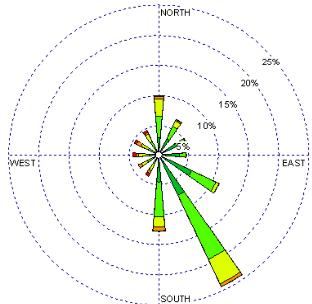
Roswell (23009) 1985-2005 November - 03-09z Average Speed - 6.03 kt
