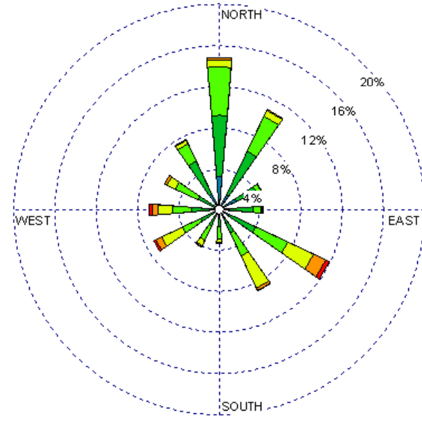
Santa Fe (23049) 1985-2005 April - 03-09z Average Speed - 7.56 kt
