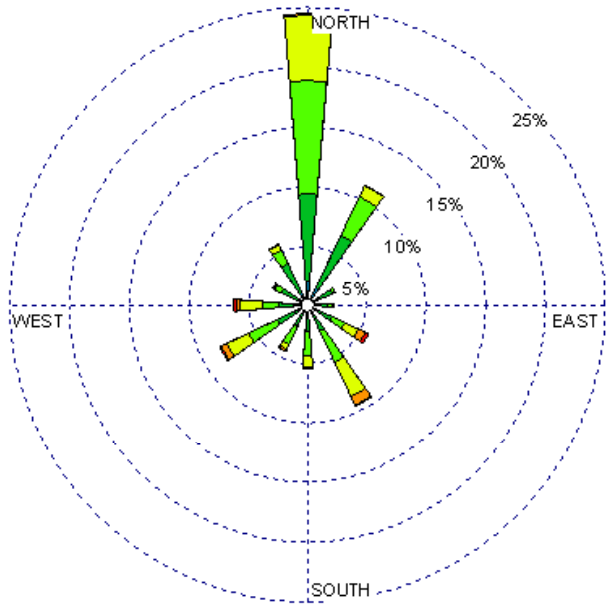
Santa Fe (23049) 1985-2005 April - 10-15z Average Speed - 7.64 kt
