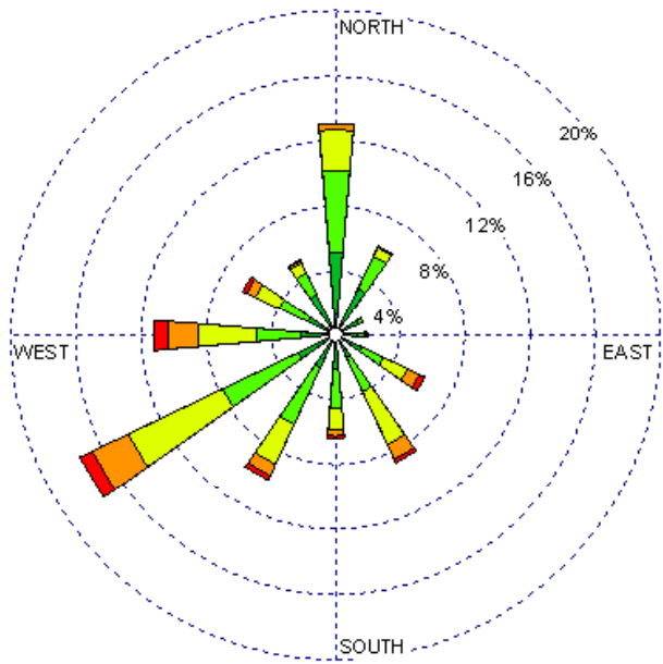
Santa Fe (23049) 1985-2005 April - All hours Average Speed - 9.98 kt
