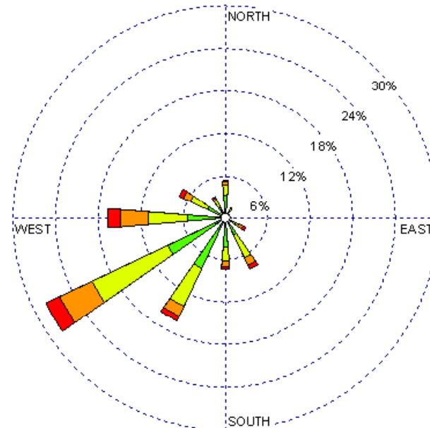
Santa Fe (23049) 1985-2005 April - 19-23z Average Speed - 13.10 kt
