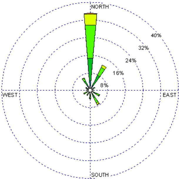
Santa Fe (23049) 1985-2005 July - 10-15z Average Speed - 6.22 kt
