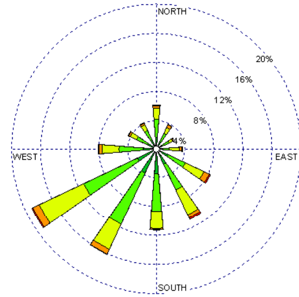
Santa Fe (23049) 1985-2005 July - 19-23z Average Speed - 10.31 kt
