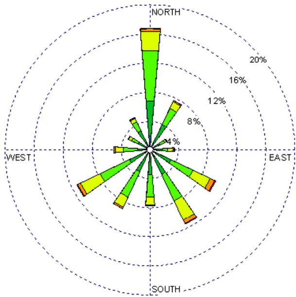
Santa Fe (23049) 1985-2005 July - All hours Average Speed - 8.30 kt
