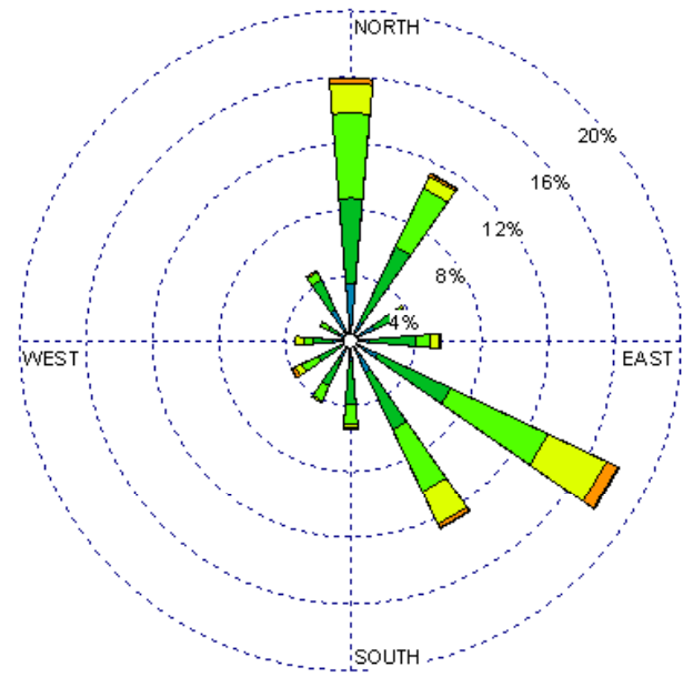
Santa Fe (23049) 1985-2005 July - 03-09z Average Speed - 7.01 kt
