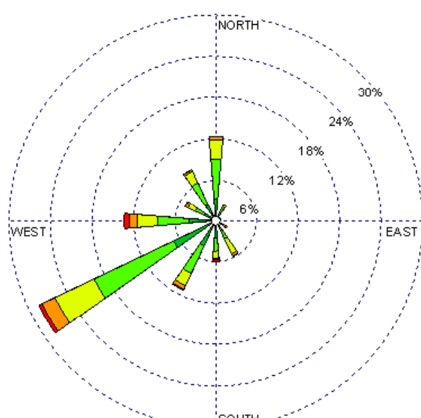
Santa Fe (23049) 1985-2005 November - 19-23z Average Speed - 9.54 kt
