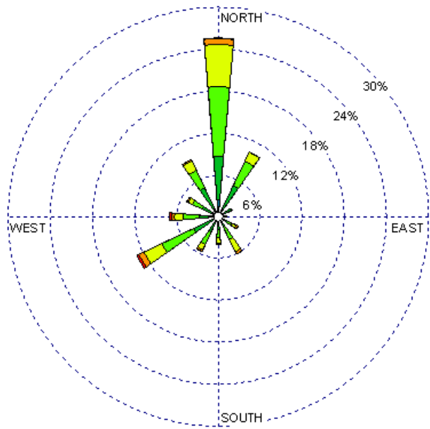
Santa Fe (23049) 1985-2005 November - All hours Average Speed - 8.21 kt
