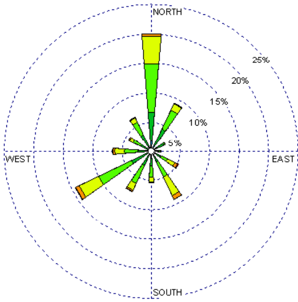
Santa Fe (23049) 1985-2005 October - All hours Average Speed - 8.30 kt
