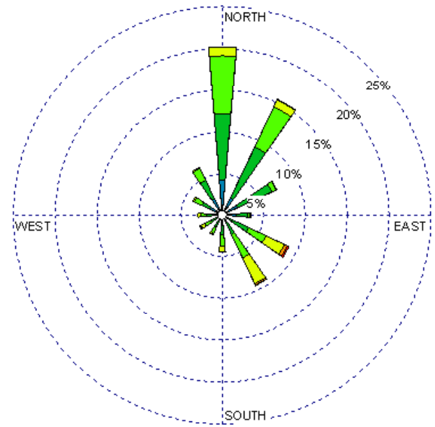
Santa Fe (23049) 1985-2005 October - 03-09z Average Speed - 6.33 kt
