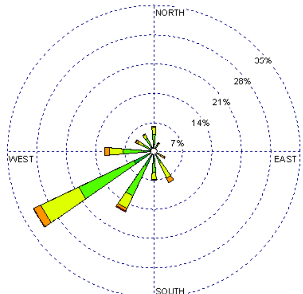
Santa Fe (23049) 1985-2005 October - 19-23z Average Speed - 10.31 kt
