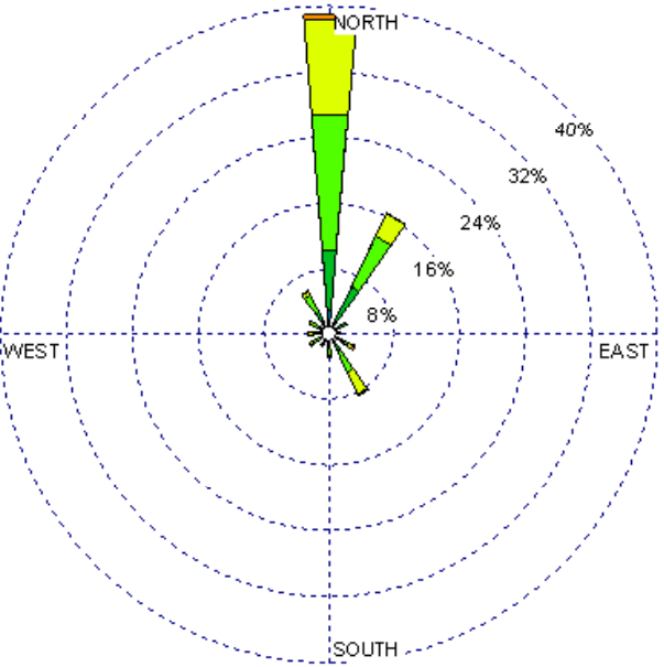
Santa Fe (23049) 1985-2005 October - 10-15z Average Speed - 7.84 kt
